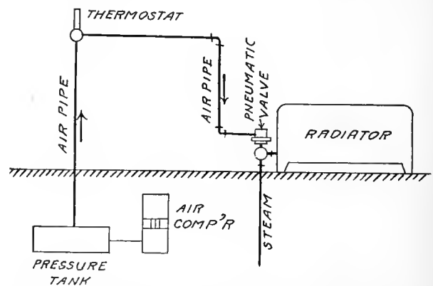
FIG. 1. DIAGRAM SHOWING THE ESSENTIAL PARTS OF A PNEUMATIC SYSTEM OF TEMPERATURE CONTROL
